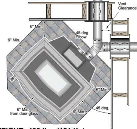
Corner Installations Through the Wall Installation
