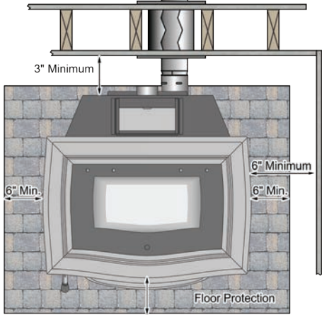
Straight Installations Through the Wall Installation
