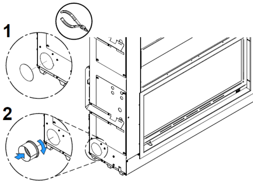
Figure 3 : Adapter installation
