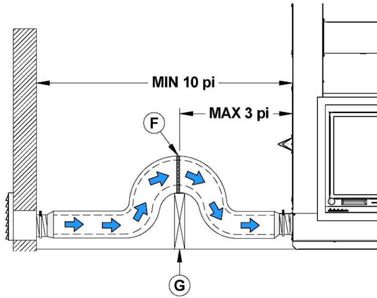
Figure 5 : P-Trap Example
