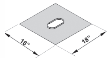
Flashing Kit
