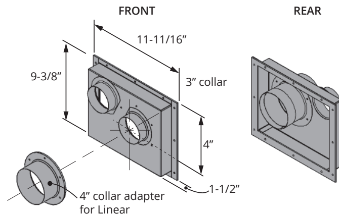
1156CLA Co-Linear Vent Adapter
