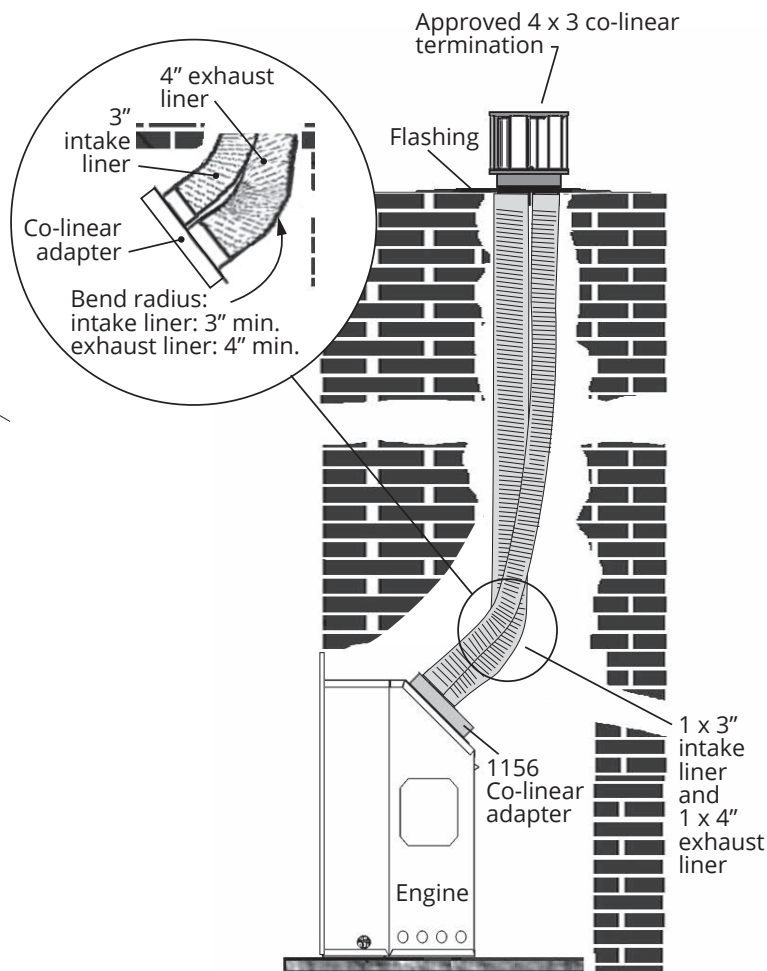
Co-linear installation into existing F/P
