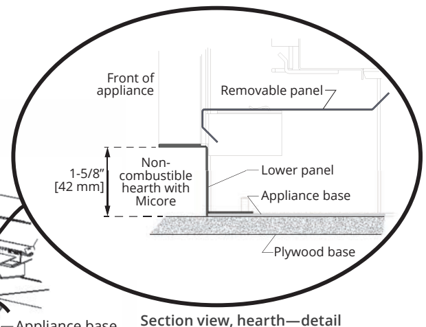
Section view, hearth—detail
