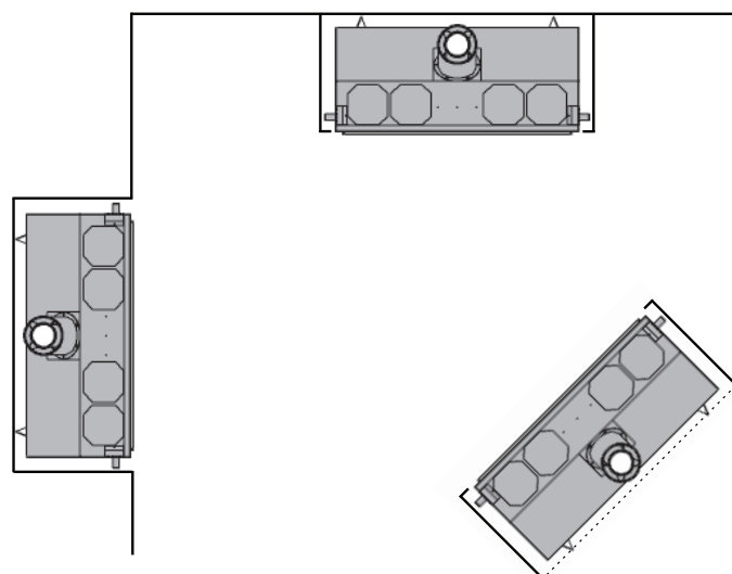
Corner Dimensions
