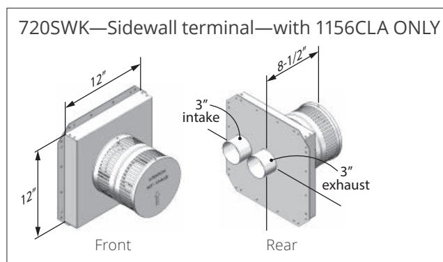
Co-Linear Terminal (typical)
