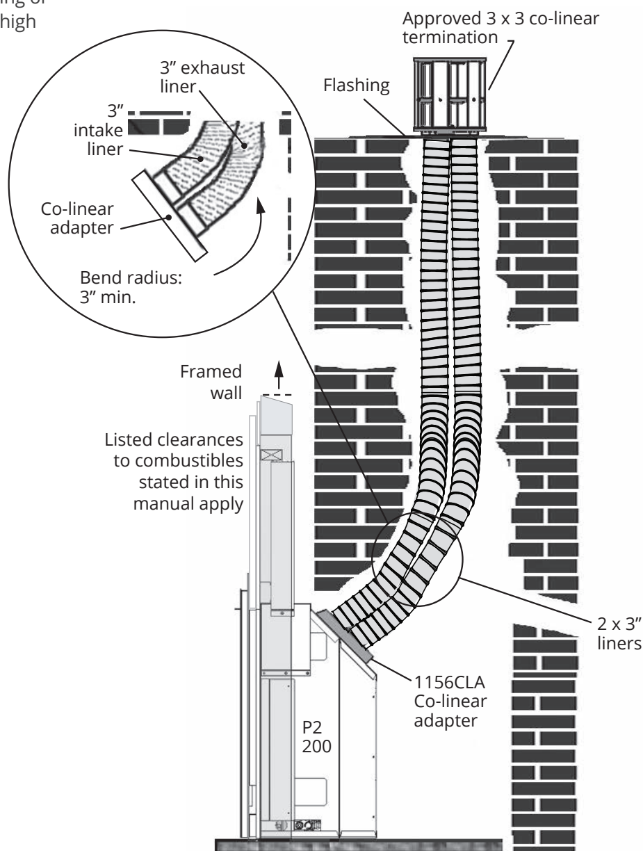
Co-linear installation on appliance partially into existing fireplace
